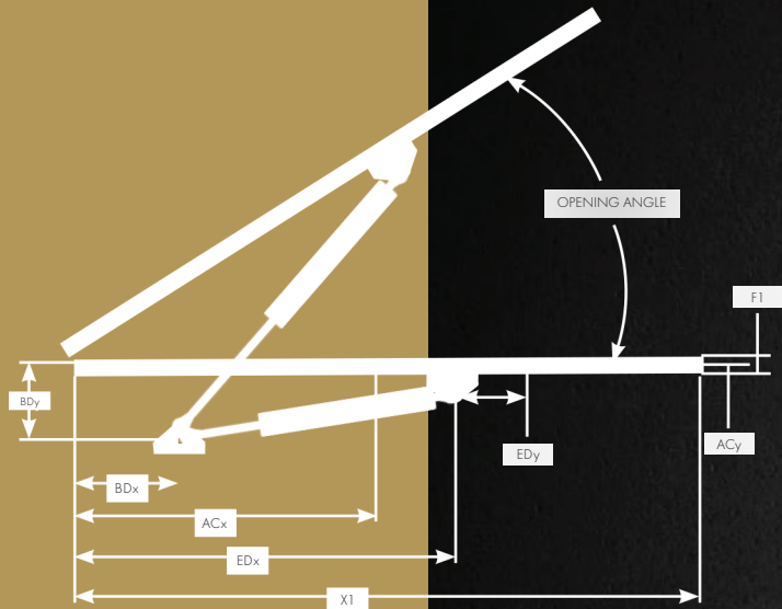
HORIZONTAL OPENING
