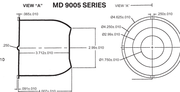
VIEW "A" MD 9005 SERIES
