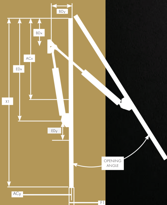
VERTICAL OPENING
